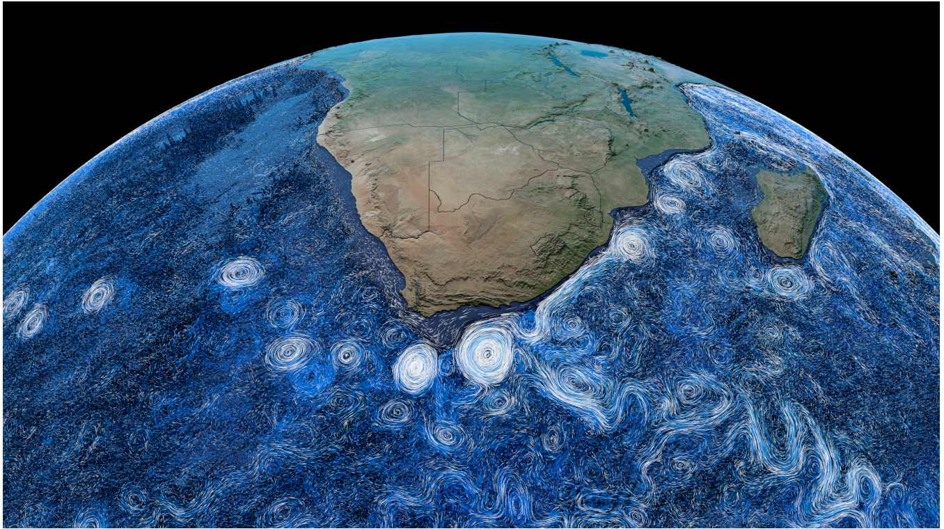
Figure 1: Perpetual Ocean 2: Western Boundary Currents
